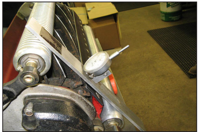
Adjustment of a Reel Mower - Photo courtesy of Doug Linde, Ph.D.
